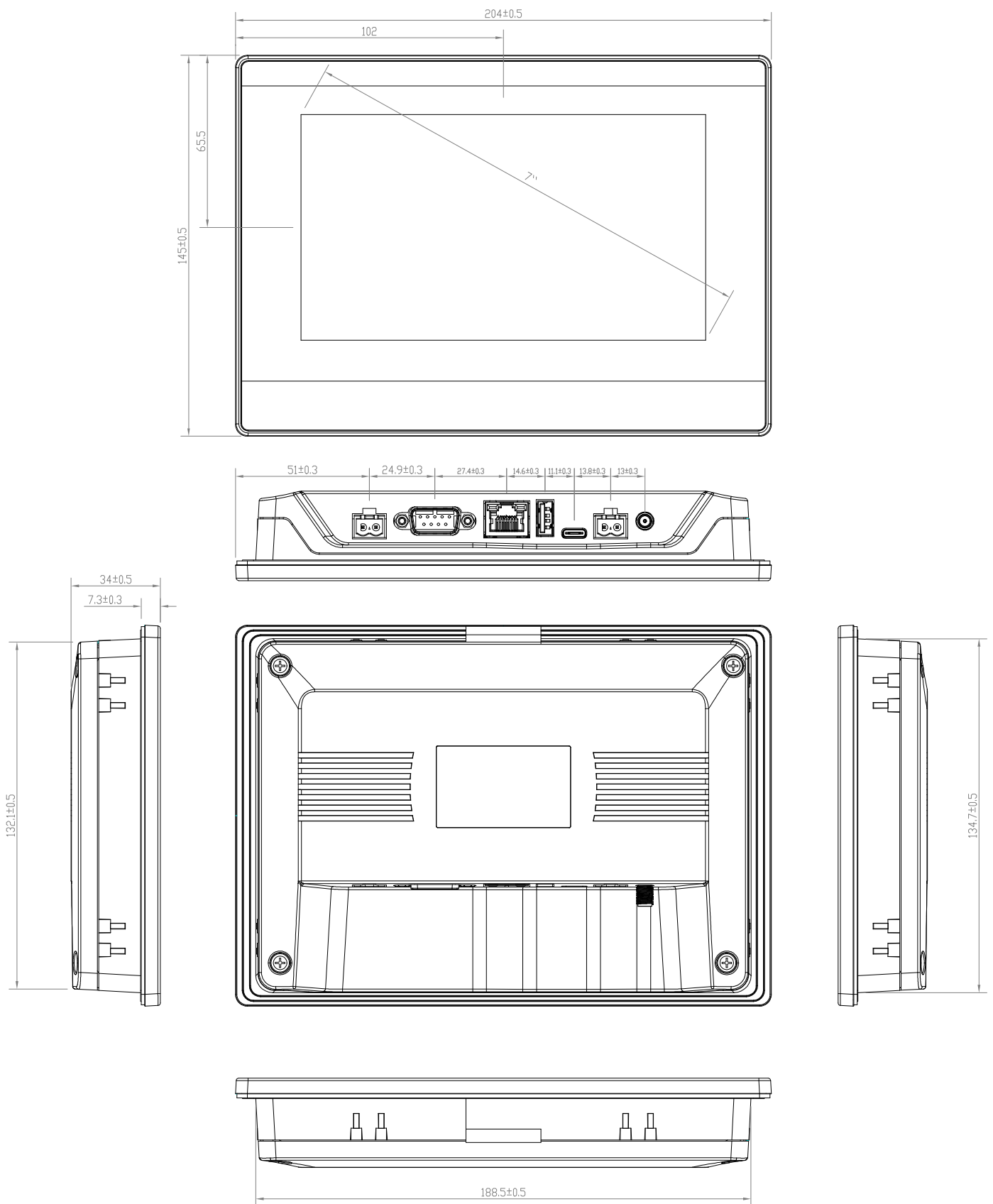
FE7070WE-4G Embedded installation opening size: 190 \times 136 MM(+1.0mm/-0.5mm)
